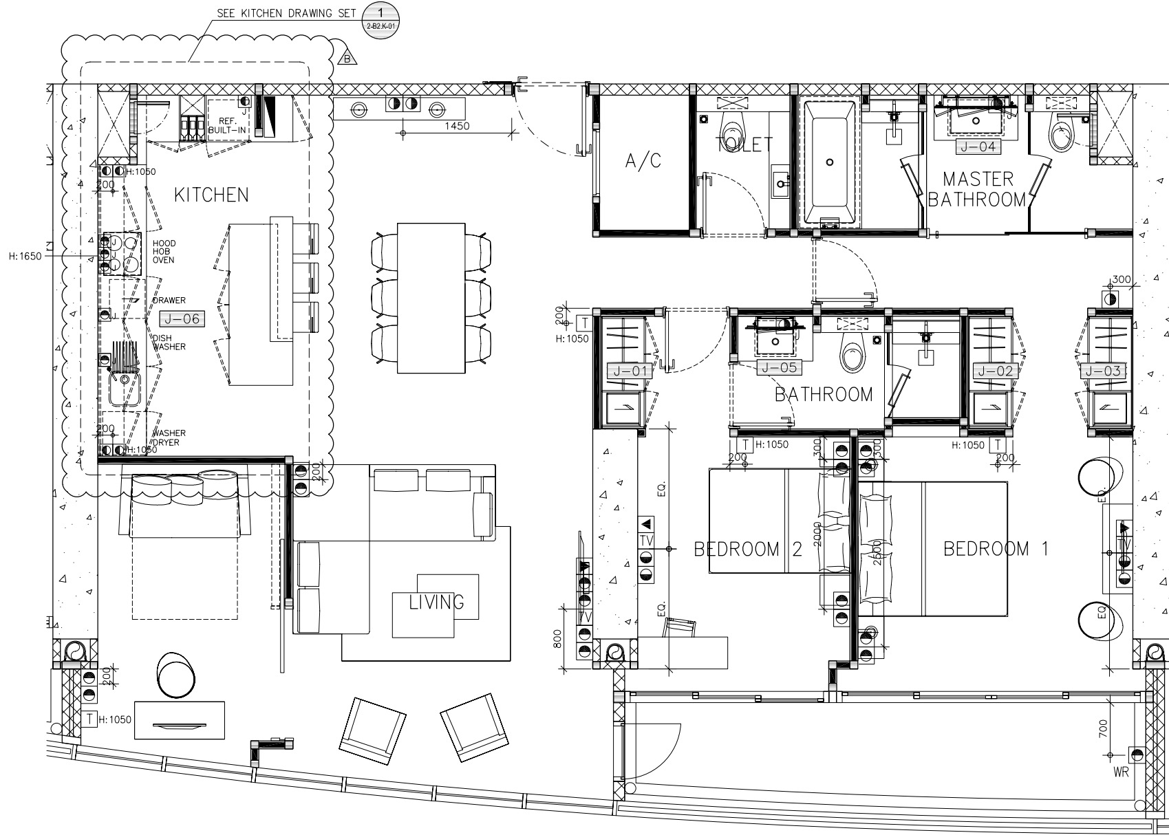
A FURNITURE & ELECTRICAL PLAN SCALE : 1:50
