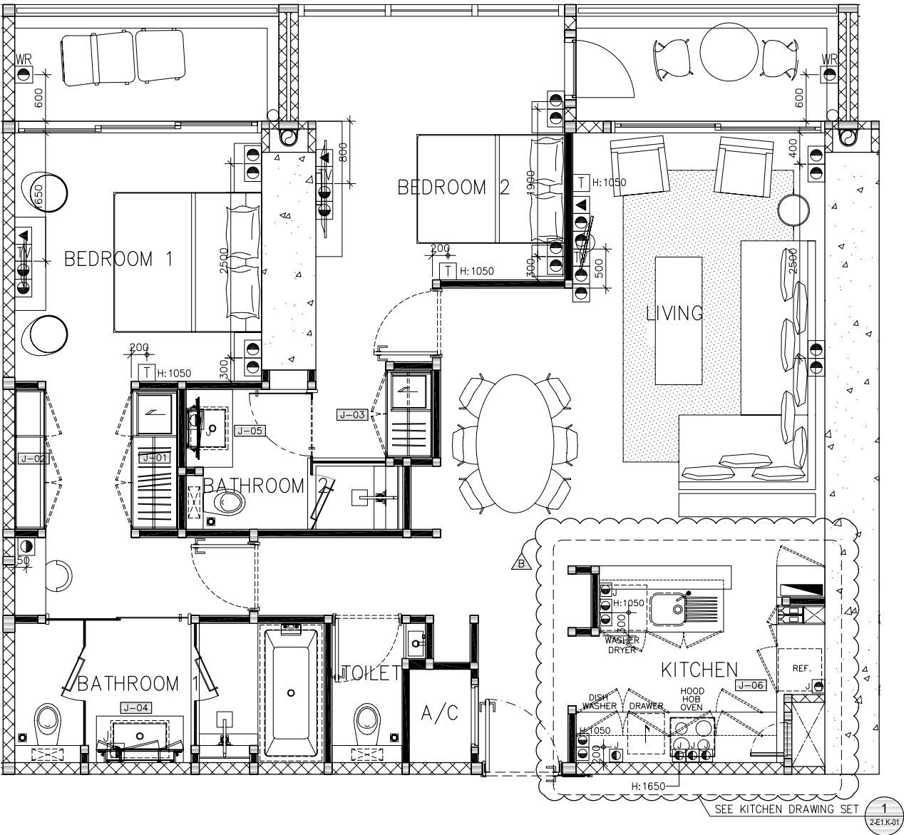
A FURNITURE & ELECTRICAL PLAN SCALE : 1 : 50
