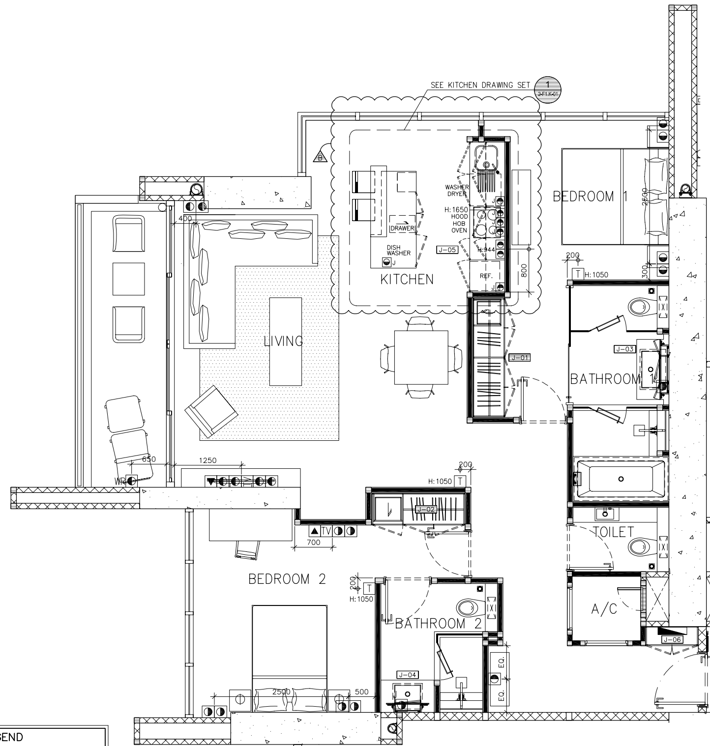
A FURNITURE & ELECTRICAL PLAN SCALE: 1:50
