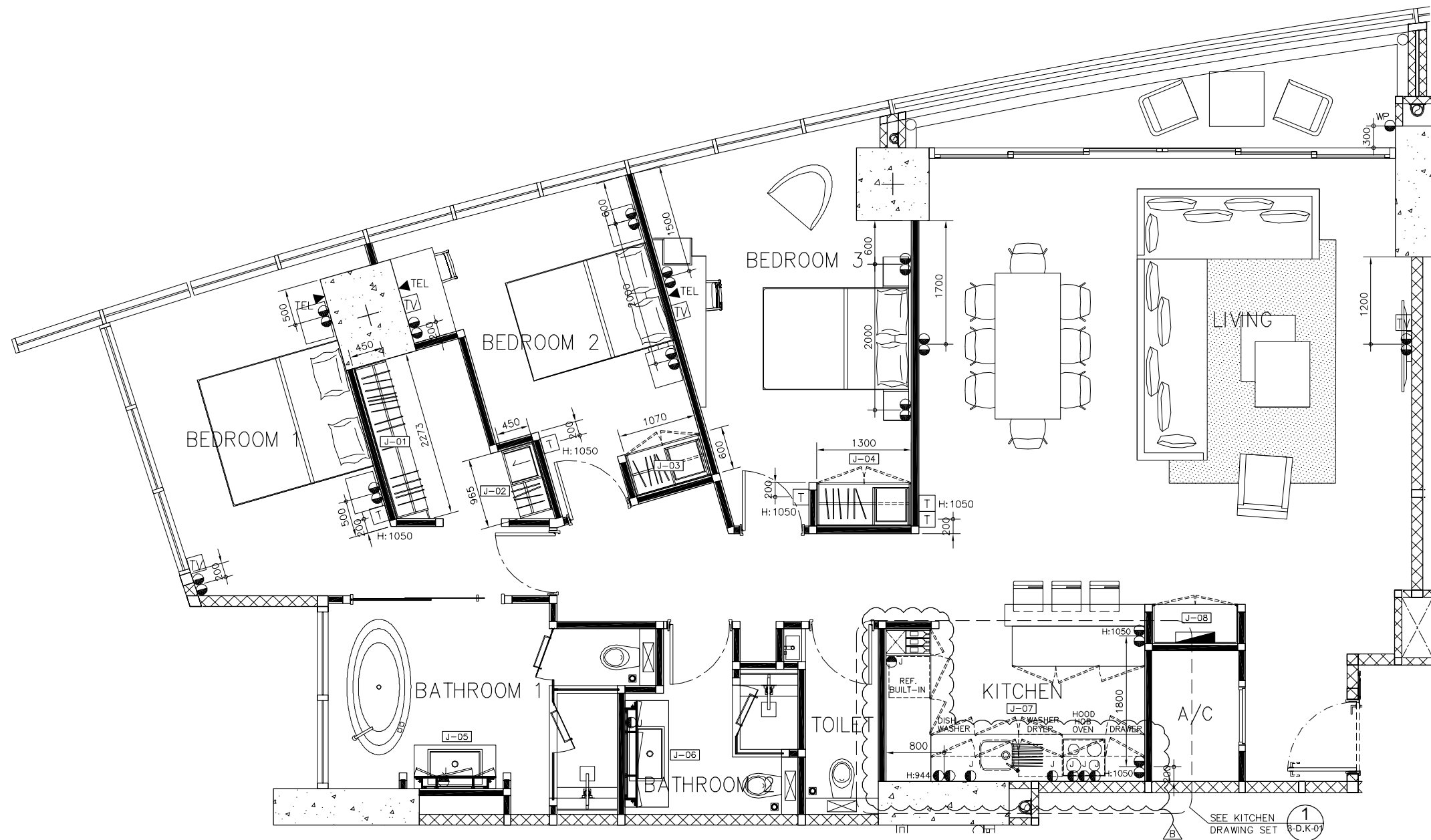
A FURNITURE & ELECTRICAL PLAN SCALE: 1:50
